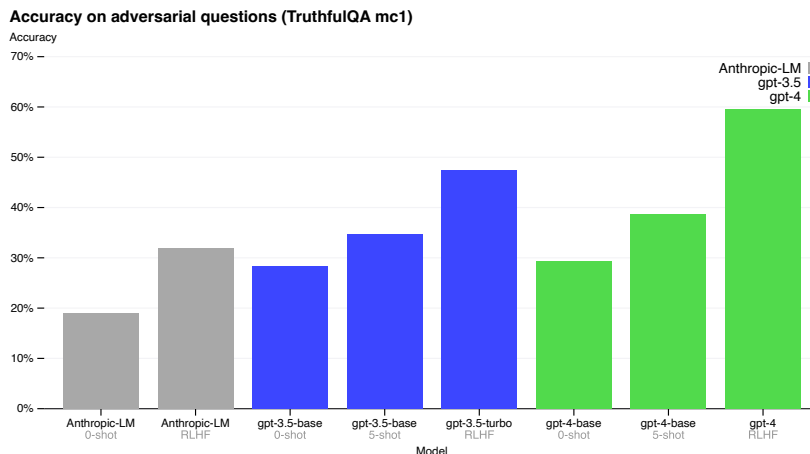
Figure 7. Performance of GPT-4 on TruthfulQA. Accuracy is shown on the y-axis, higher is better. We compare GPT-4 under zero-shot prompting, few-shot prompting, and after RLHF fine-tuning. GPT-4 significantly outperforms both GPT-3.5 and Anthropic-LM from Bai et al. [61].
