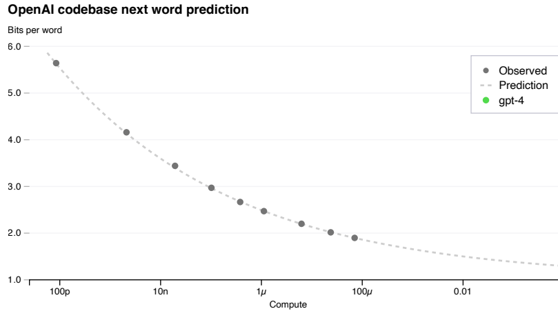
Figure 1. Performance of GPT-4 and smaller models. The metric is final loss on a dataset derived from our internal codebase. This is a convenient, large dataset of code tokens which is not contained in the training set. We chose to look at loss because it tends to be less noisy than other measures across different amounts of training compute. A power law fit to the smaller models (excluding GPT-4) is shown as the dotted line; this fit accurately predicts GPT-4’s final loss. The x-axis is training compute normalized so that GPT-4 is 1.
