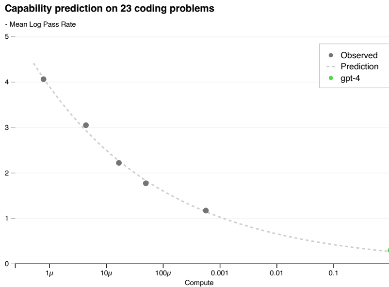
Figure 2. Performance of GPT-4 and smaller models. The metric is mean log pass rate on a subset of the HumanEval dataset. A power law fit to the smaller models (excluding GPT-4) is shown as the dotted line; this fit accurately predicts GPT-4’s performance. The x-axis is training compute normalized so that GPT-4 is 1.
